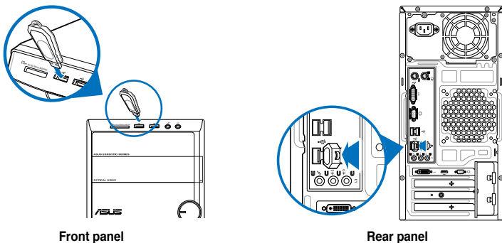
Front panel
